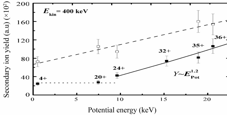
Fig. 1 Sputtering yields increase as a function of the potential energy when Pb q+ impact on SiO 2 and Au surfaces.
