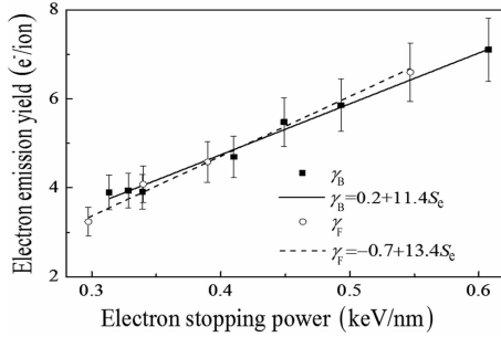
Fig. 1 Electron stopping power at the entrance and exit surfaces dependence of the SEE yield from the forward and backward directions.
