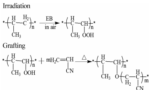
Fig. 1 Grafting progress.
