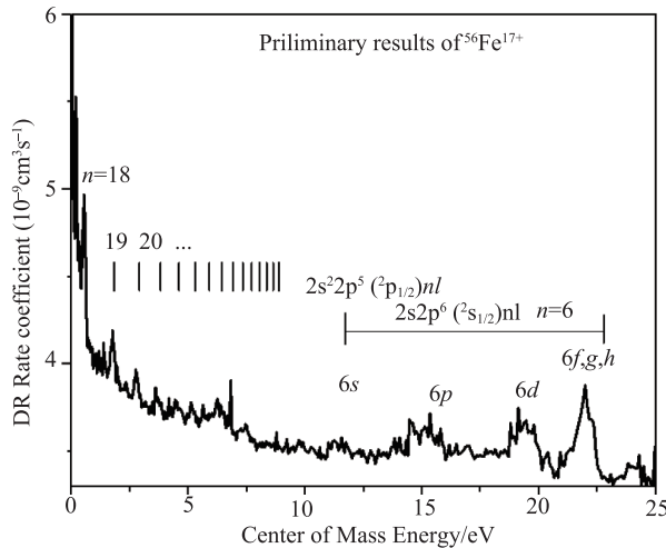
Fig. 1 (color online) The experimental DR rate coefficients for F-like ^{56}\text{Fe}^{17+} ions versus the collisional energy between electron and the ion beam in the c.m. frame. The DR resonances involve \Delta n = 0 transition. The observed DR channels are \text{Fe}^{17+} (2s^2 2p^5 [^2P_{3/2}]) + e^- \rightarrow \text{Fe}^{16+} (2s^2 2p^5 [^2P_{1/2}] nl) (n = 18, \dots) and \text{Fe}^{17+} (2s^2 2p^5 [^2P_{3/2}]) + e^- \rightarrow \text{Fe}^{16+} (2s^2 2p^6 [^2S_{1/2}] nl) (n = 6, \dots) respectively, which are indicated by vertical bars.
