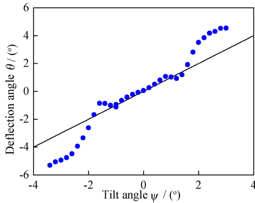
Fig. 1 (color online) The dependence of the deflection angle on the capillary tilt angle for 1.5 keV electrons passing through a plate capillary. The solid line represents \psi = \theta .
